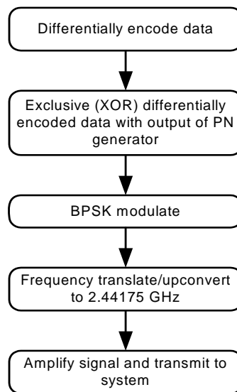
Figure 6 — Transmitter data encoding and transmission process
