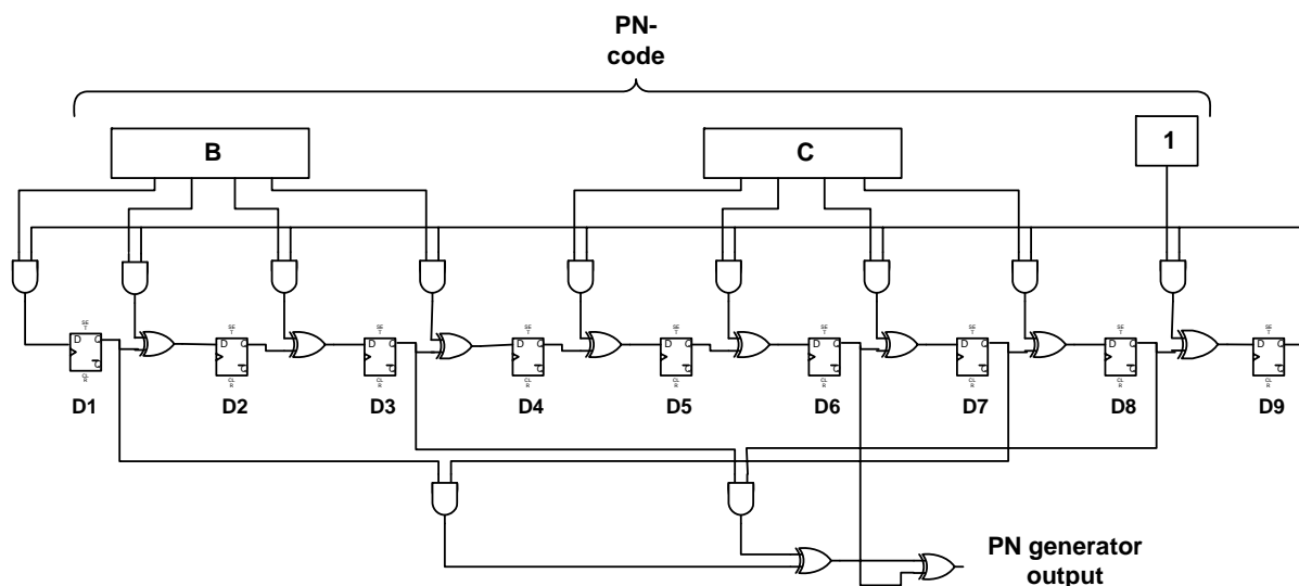
Figure 5 — eSeal transmitter PN generator
