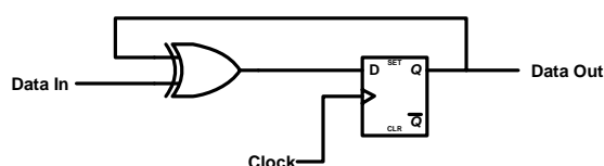
Figure 4 — Example of differential encoding circuit
